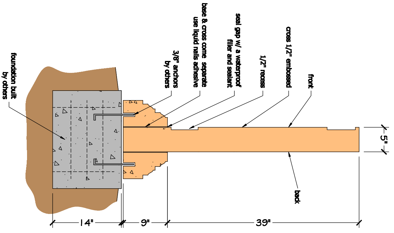
3 Section
